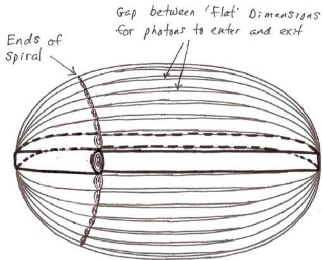
Figure 3. Geometric rendition of a fundamental particle where the cross-section of the spiral branes is shown.
