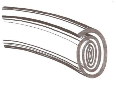
Figure 1. Geometric rendition of CWEP folds in a Fibonacci spiral cross-section.
